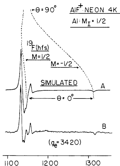
Figure 5. Simulated (A) and experimental (B) ESR spectra of \text{AlF}^+ in neon matrix for the Al M_I = 1/2 transition is presented. The dashed curves show the \theta vs. H_{\text{RES}} dependence. An intense off-angle line is observed for the lower field ^{19}\text{F} component that overlaps the normally dominant \theta = 90^\circ (perpendicular transition). See Figure 4 and Table I for exact line positions and magnetic parameters employed.
