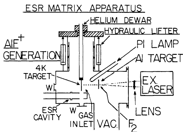
Figure 1. ESR matrix apparatus used for generating AlF from laser sputtering an aluminum target under F_2(g) flow conditions. AlF^+ is formed during neon deposition by photoionization from the open-ended neon resonance lamp (16.8 eV) labeled "PI".
